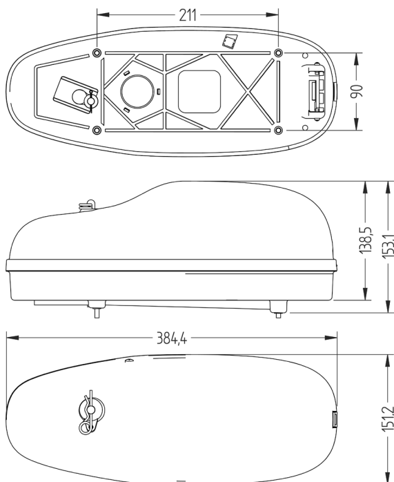
Figure 6 Illustration - FB-60 float free bracket dimensions
