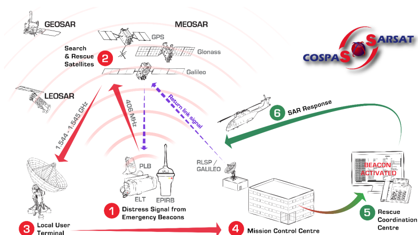
Figure 2 Illustration - signal detection
