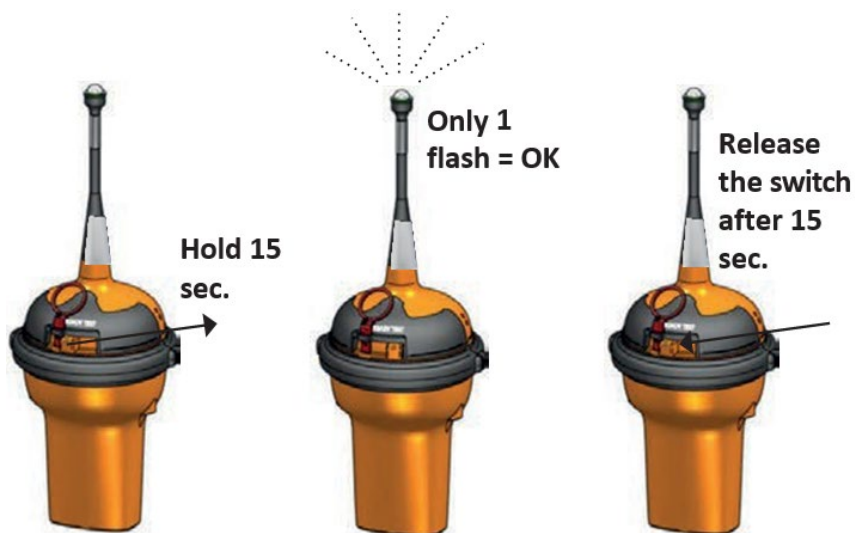
Figure 9 Illustration – Normal self-test
