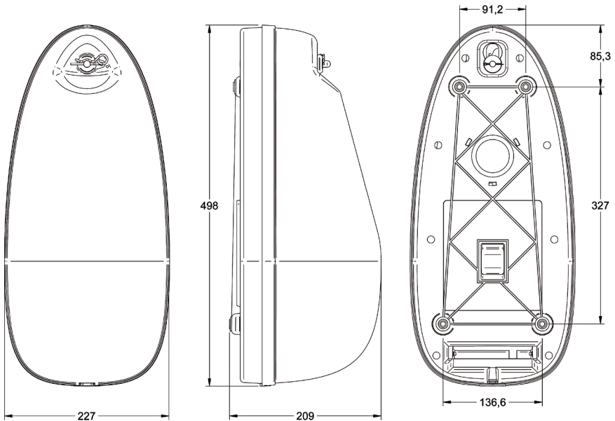
Figure 4 Illustration - FB-6 float free bracket dimensions
