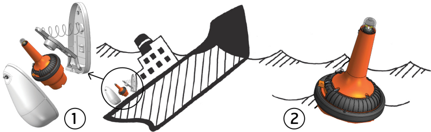
Figure 5 Illustration - automatic operation of a FB-6 float free bracket
